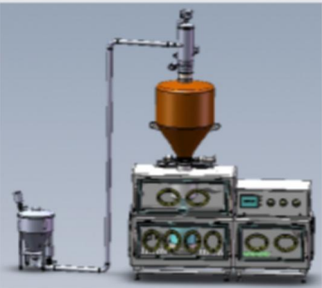
Integration isolation system with filtration, drying, weighing and filling process
